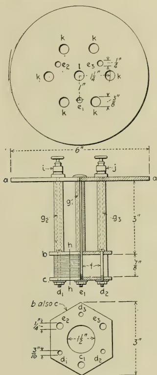
FIG. 174.—Heating Coil for K. & S. Fusing-Point Tester.
